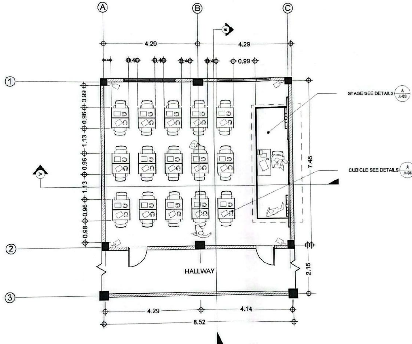
FLOOR PLAN SCALE 1 : 75
