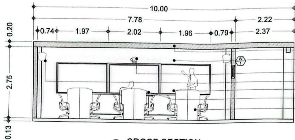
CROSS SECTION SCALE 1 : 60 M.
