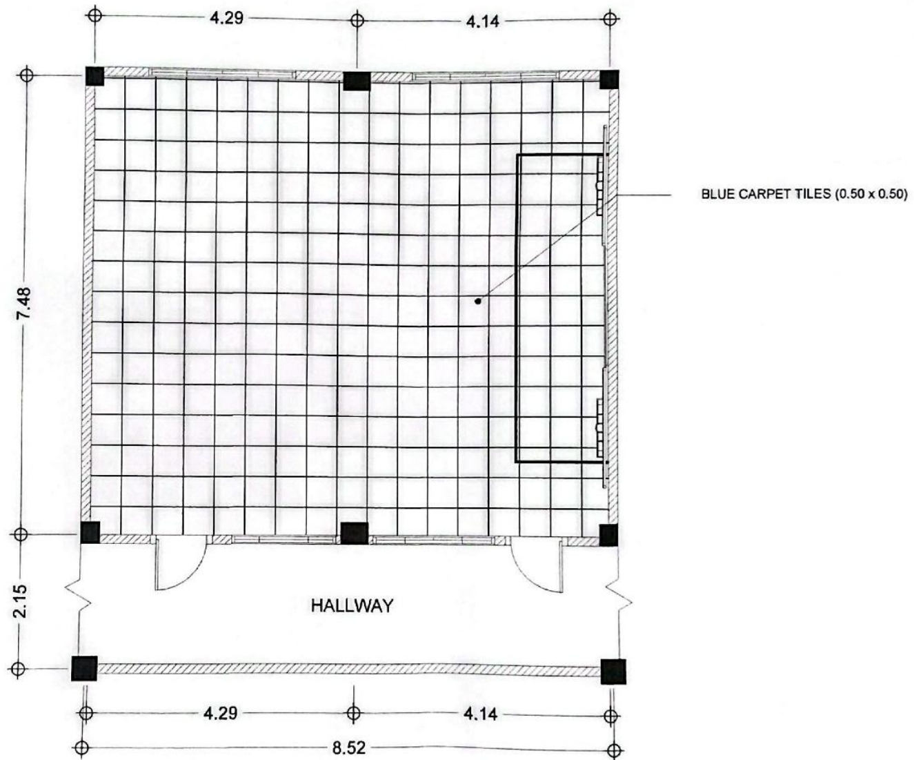
TILE LAYOUT PLAN SCALE 1 : 60
